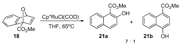
Scheme 4. Isomerization of oxabenzonorbornadiene 18 .
