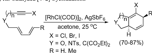
Scheme 2. Transition-metal-catalyzed cycloaddition reactions of alkynyl halides.
