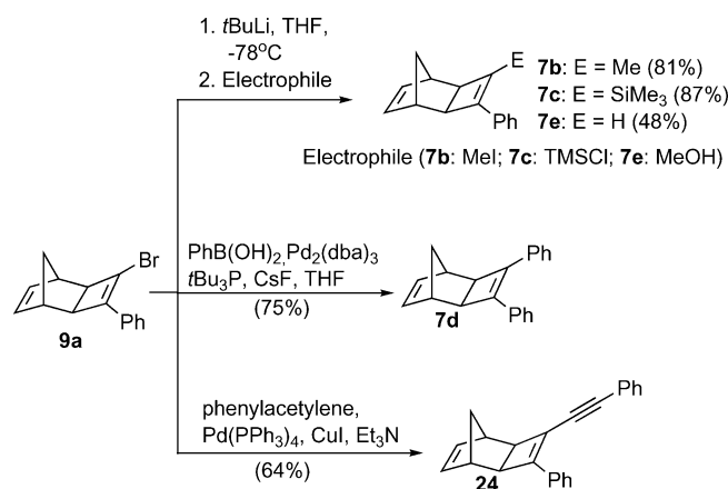
Scheme 6. Functionalization of cycloadduct 9a .
