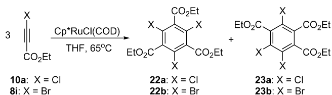
Scheme 5. Cyclotrimerization of alkynyl halides 10a and 8i .
