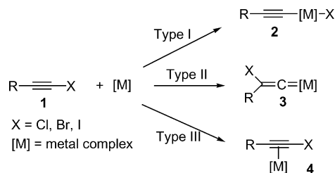
Scheme 1. Potential reactivity pathways of alkynyl halides in transition-metal-catalyzed reactions.
