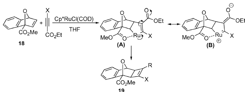
Scheme 3. Possible explanation of regioselectivity.
